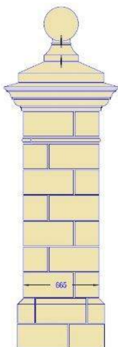
Type A 665mm With Plain Quoin body
